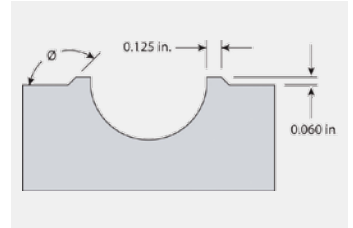
Figure 7: A rib is added to the tool design. The rib follows the contours of the mold cavity.
