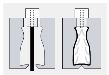
Figure 2: In extrusion blow molding, a molten tube of plastic is extruded into a mold cavity and inflated with compressed air
