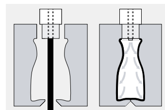
Figure 5: Continuous extrusion blow molding. The parison is extruded through a die (left), and the mold closes on the tube of plastic. The parison is then inflated (right) to force the plastic to the contours of the tool.
