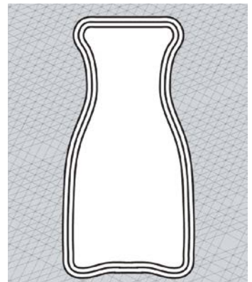
Figure 12: Increasing the number of contour passes reduces porosity and improves part quality.
