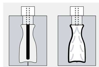
Figure 6: Intermittent extrusion blow molding. The parison is extruded within the mold cavity (left) and inflated with air pressure (right).
